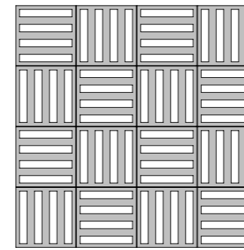
laying scheme 1
